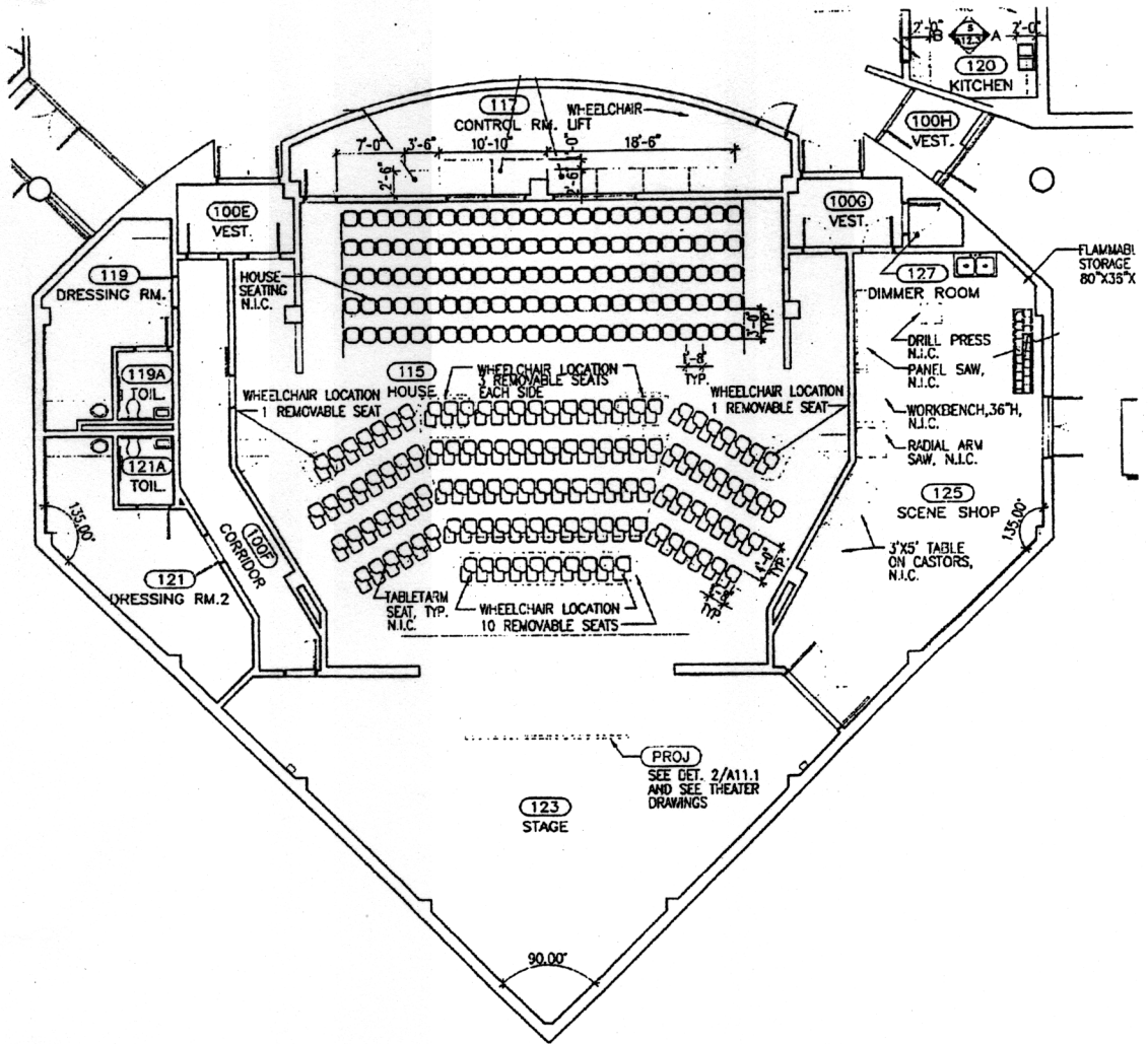
2 FIRST FLOOR FURNITURE AND EQUIPMENT PLAN
