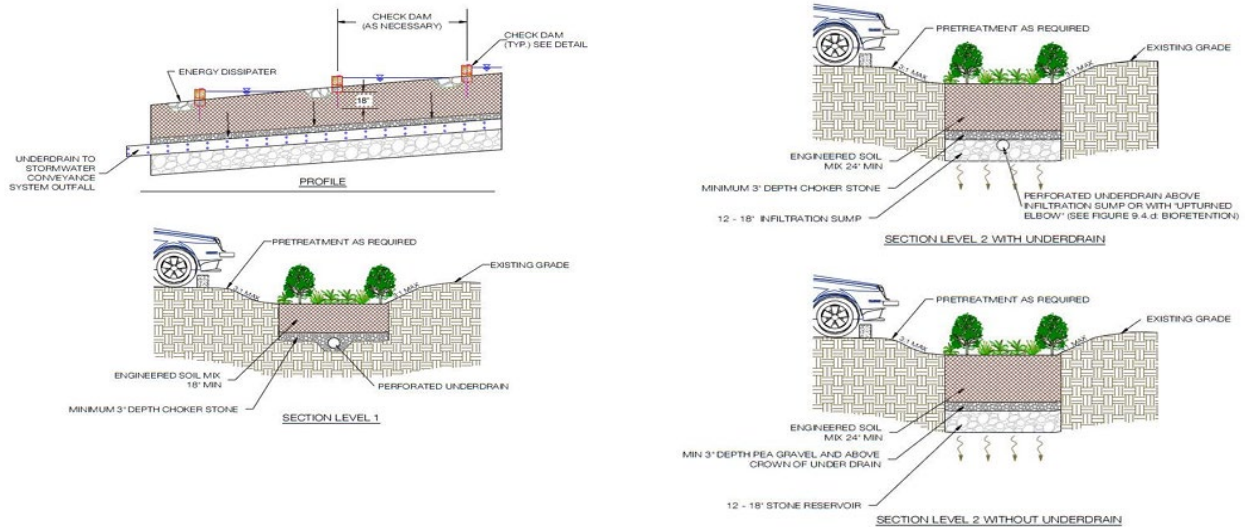
Figure 10: Typical Dry Swale Details
