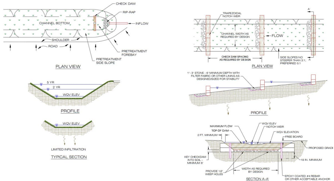
Figure 8: Typical Grass Channel Details
